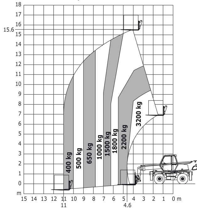
Machine on tyres with forks Metric
